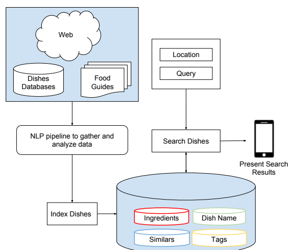
Figure 1: Architecture of Appetitoso.
