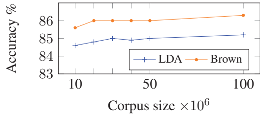
Figure 4: Clustering results
