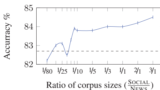
Figure 2: Oversampling results
