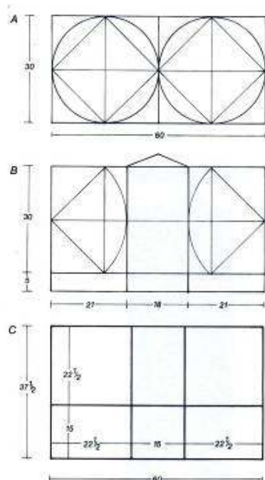
Fig. 12. Reconstruction of Vingboons' system for Vechtvliet, 1665
